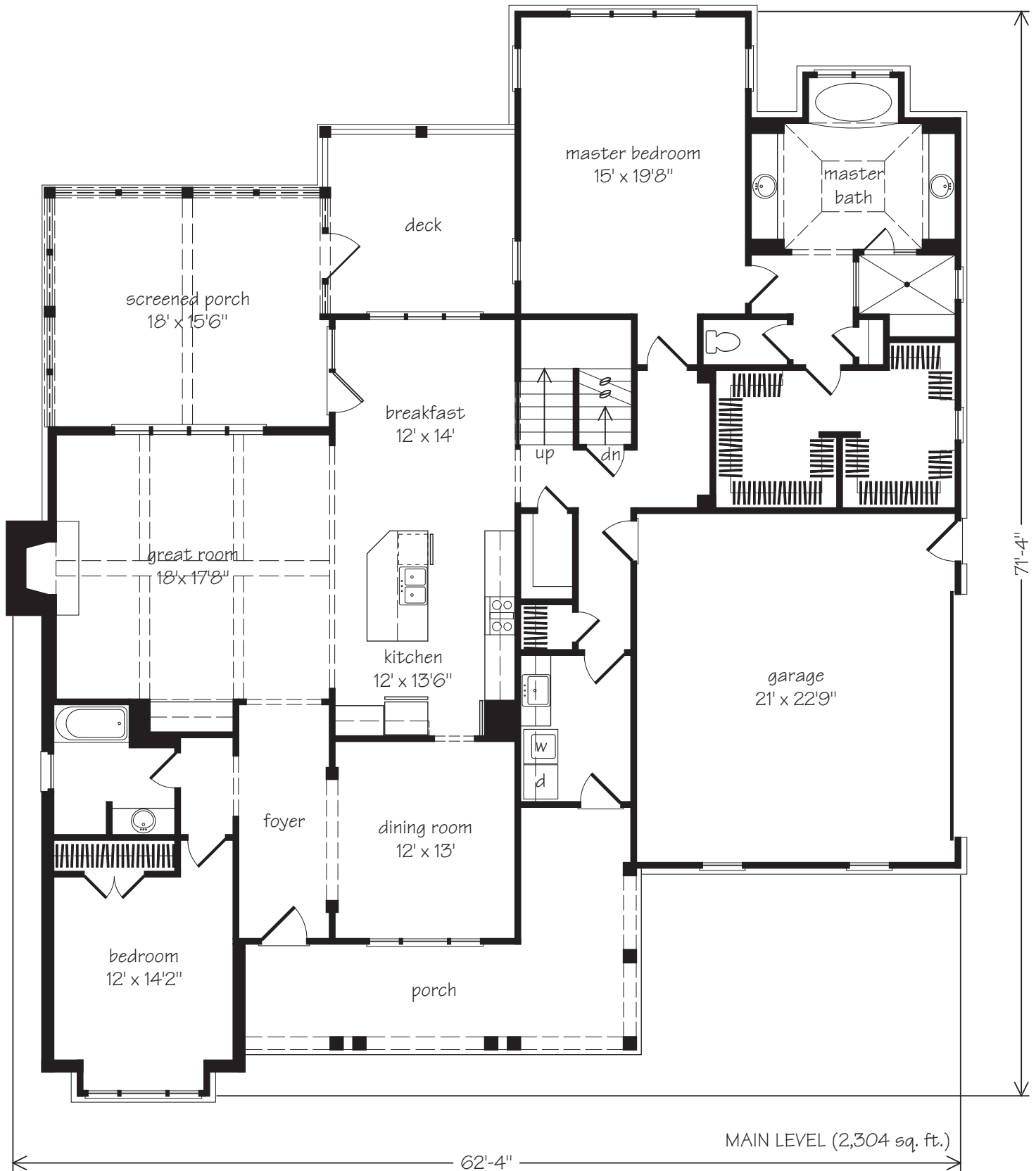
#1440 Bucknell Place: Main Level Floor Plan
