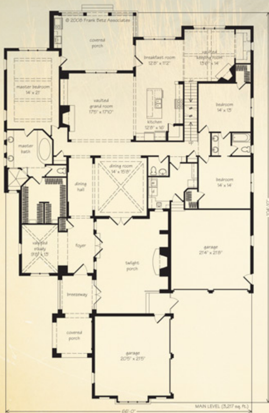
#1654 Falkirk Ridge: Main Level Floor Plan
